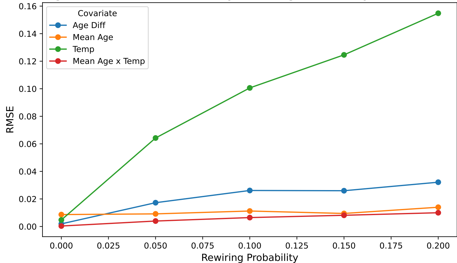
Exogenous Coefficient RMSE by Rewiring Probability (13 nodes): ER
