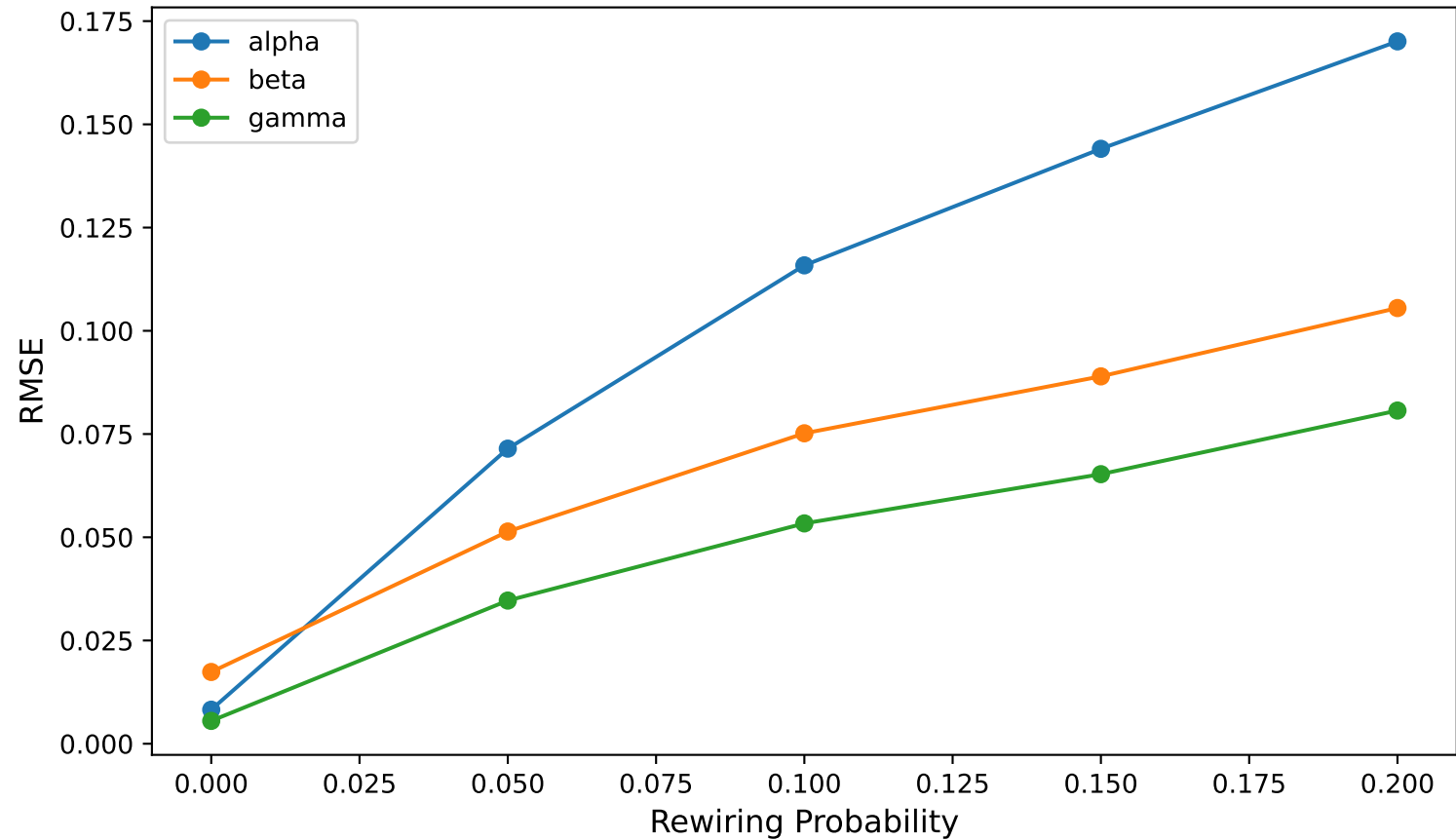
RMSE by Rewiring Probability (13 nodes): ER
