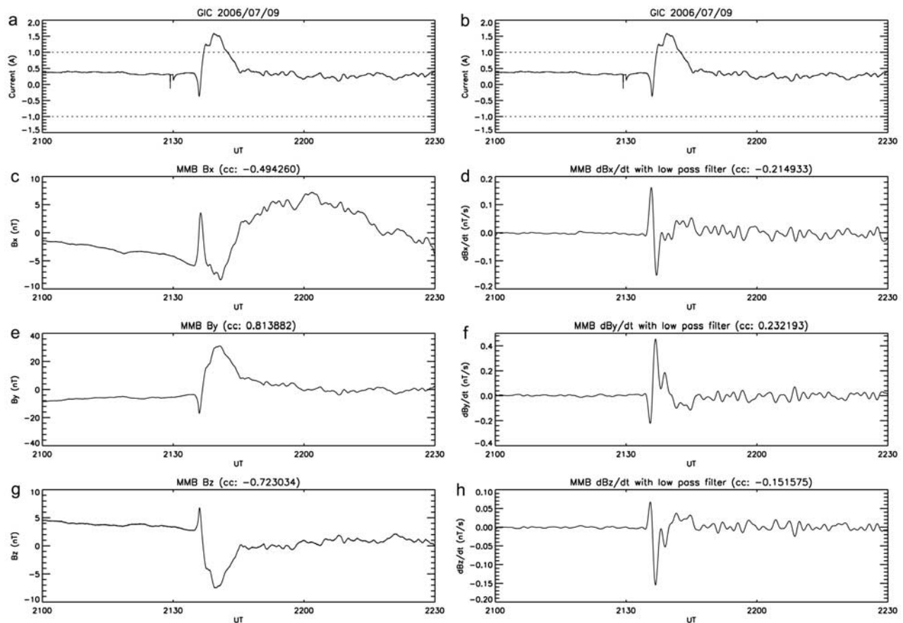
Figure 3. Same as Figure 2, except for a (a and b) GIC event associated with an SI at 2134UT on 9 July 2006 and the (c) Bx, (e) By, (g) Bz, (d) dBx/dt, (f) dBy/dt, and (h) dBz/dt components of geomagnetic variations at MMB.
