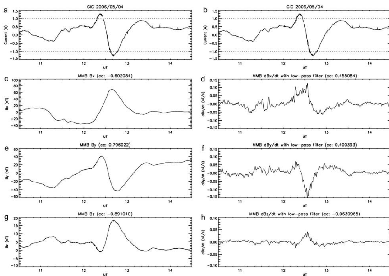
Figure 4. Same as Figure 2, except for a (a and b) GIC event associated with a middle-latitude positive bay on 4 May 2006 and (c) Bx, (e) By, (g) Bz, (d) dBx/dt, (f) dBy/dt, and (h) dBz/dt components of geomagnetic variations at MMB.
