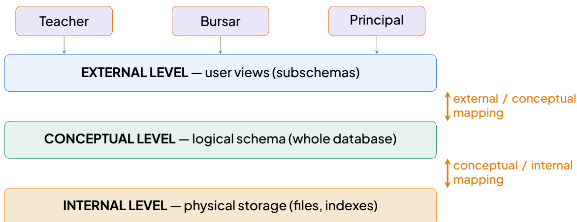
The ANSI-SPARC three-level architecture with its two mappings.
