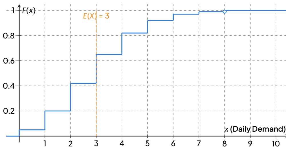
Cumulative distribution function F(x) = P(X \leq x) for the daily demand (Poisson \lambda = 3 ).
