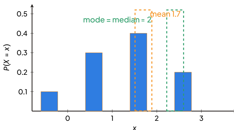
Bar chart of the distribution with the mean (orange dashed line) and the common value of the mode and median (green dashed line).
