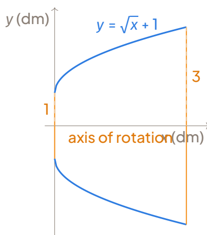
Profile of the pot and the solid generated by rotation about the x -axis.
