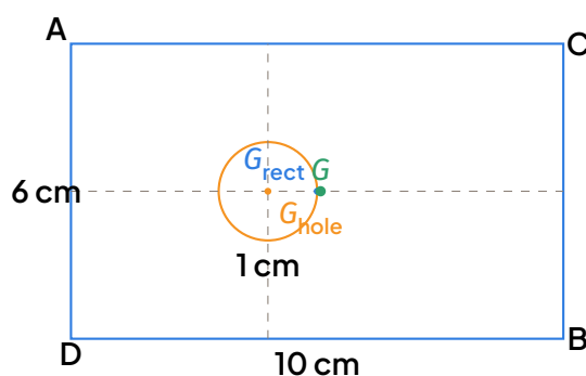
Rectangle with a circular hole. The hole is treated as negative area.
