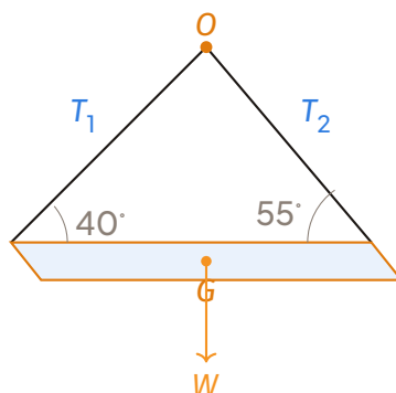
Free-body diagram of the loaded tray suspended by two strings.
