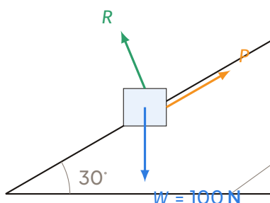
Free-body diagram of the block on the smooth inclined plane.
