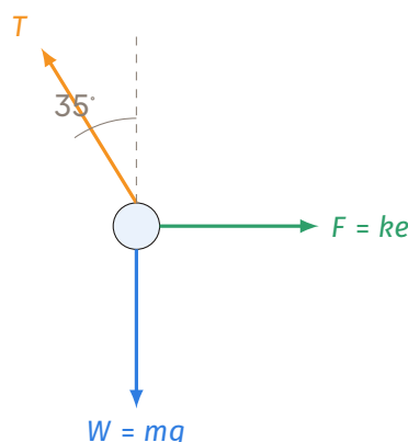
Free-body diagram: weight, tension, spring force.
