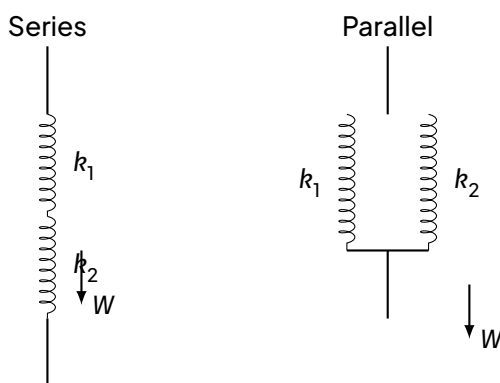
Springs in series (left) and in parallel (right) carrying the same load W . Extensions add in series; loads share in parallel.
