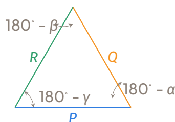
Force Triangle
