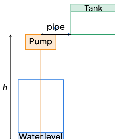
Pump raising water from a well to an overhead tank with ejection speed v .
