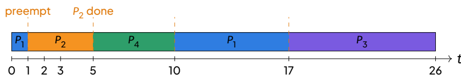
Gantt chart for SRTF. P_1 is preempted at t = 1 when the shorter job P_2 arrives.
