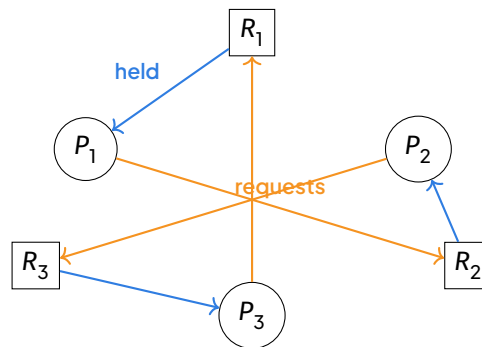
Resource Allocation Graph: assignment edges R_i \rightarrow P_j (blue) and request edges P_i \rightarrow R_j (orange).
