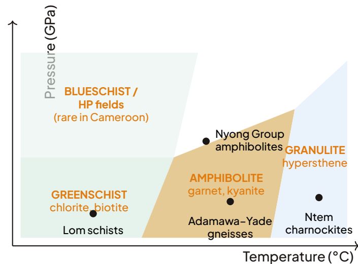
Schematic pressure-temperature (P-T) diagram of metamorphic facies, with typical Cameroonain terrains placed in their approximate fields.
