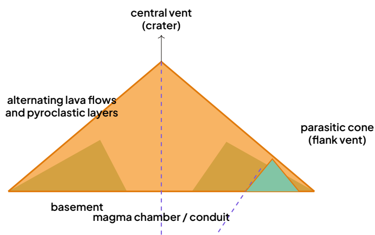
Schematic cross-section of a CVL stratovolcano (e.g. Mount Cameroon).
