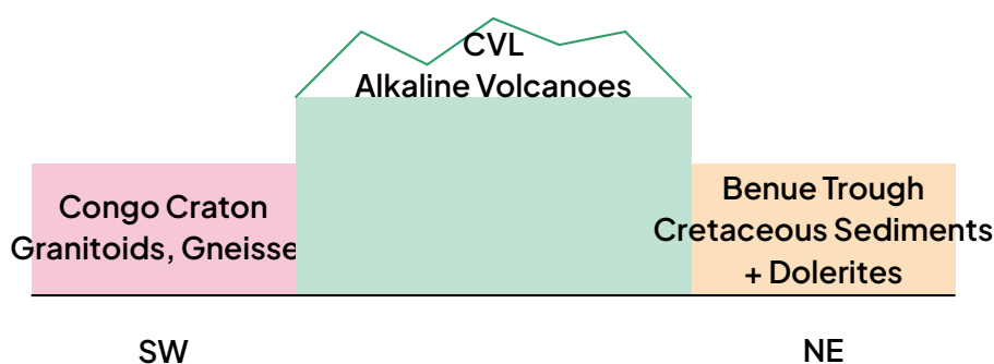
Schematic SW-NE cross-section across Cameroon showing the three igneous provinces.
