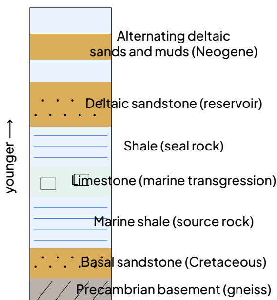
Schematic stratigraphic log of the Douala Basin, showing the sandstone–shale–limestone alternations above the Precambrian basement and the petroleum roles of each unit.
