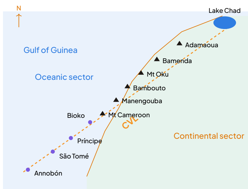
Simplified map of the Cameroon Volcanic Line: a SW–NE alignment of volcanic centres crossing from oceanic crust (islands) onto continental crust (mainland massifs) up to the Lake Chad basin.
