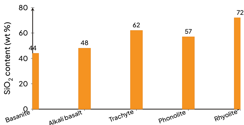
Typical silica contents of CVL lavas, showing the alkaline differentiation trend from basanite (about 44 % SiO 2 ) to rhyolite (over 70 % SiO 2 ).
