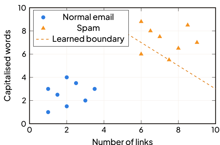
A supervised classifier: the model has learned a boundary (dashed line) separating two classes of labelled examples.
