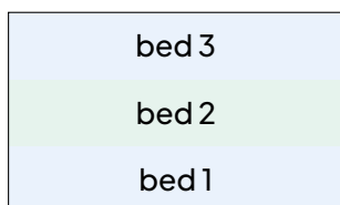
(a) Horizontality
