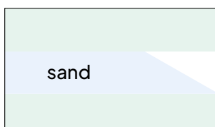
(b) Pinch-out
