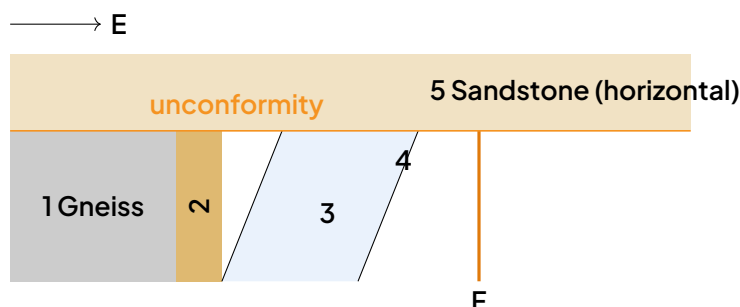
Schematic E–W cross-section: tilted Units 2–4 and the fault F are truncated by the unconformity and sealed by the horizontal Carboniferous sandstone (Unit 5).
