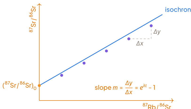
Schematic Rb–Sr isochron diagram. Cogenetic samples define a straight line whose slope gives the age and whose intercept gives the initial strontium isotope ratio.
