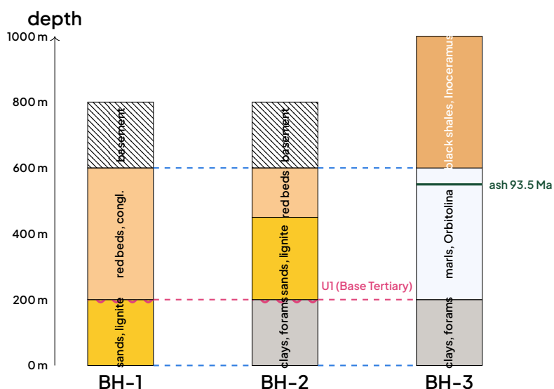
Correlation panel (fence diagram) of the three boreholes. Dashed lines: correlated unit boundaries; U1 = Base Tertiary unconformity.
