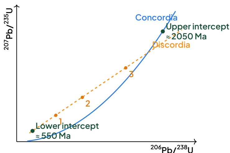
Concordia diagram: the three discordant zircon analyses define a Discordia line intersecting the Concordia curve at two points.
