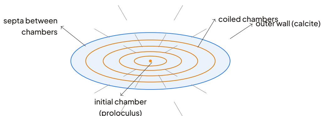
Median section through the coin-shaped test of Nummulites (Eocene), showing the planispiral arrangement of chambers around the initial chamber (proloculus).
