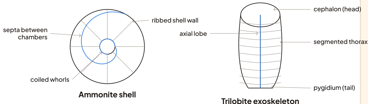
Two classic body fossils: the coiled, chambered shell of an ammonite (left) and the three-lobed, segmented exoskeleton of a trilobite (right).
