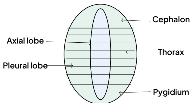
Labelled sketch of a trilobite (dorsal view).
