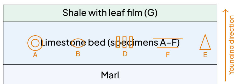
Simplified log of the fossiliferous bed at Figuil showing the position of the specimens.
