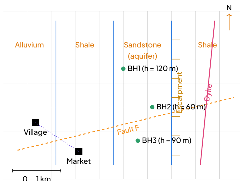
Simplified geological map of the Nkwen–Bafut area. Scale: 1 cm = 0.5 km (1:50 000). Grid squares are 1 cm × 1 cm. The sandstone unit is the water-bearing bed (aquifer).
