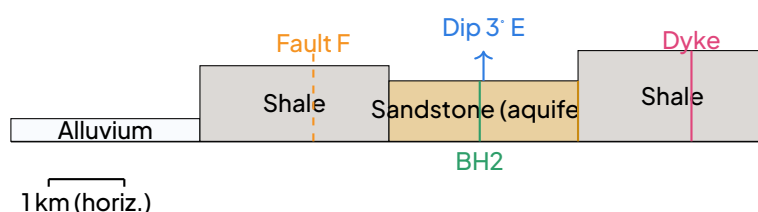
Schematic geological cross-section (west-east through BH2) with no vertical exaggeration. The gentle eastward dip of the sandstone aquifer is shown.
