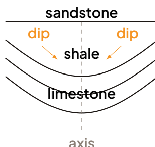
Cross-section of a syncline: mirror-image repetition, dips converge towards the axis.
