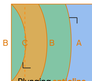
Plunging anticline oldest (C) in core plunges North
