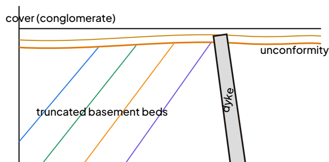
Angular unconformity with a cross-cutting dyke
