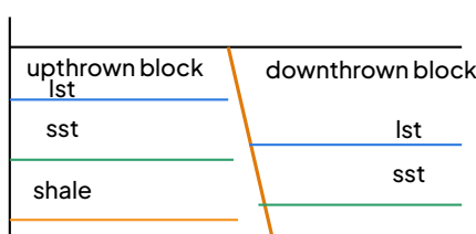
Section: normal fault, throw to the east
