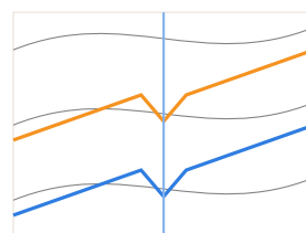
Dipping beds contacts make V's in the valley
