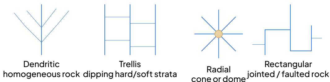
The four fundamental drainage patterns and their geological significance.
