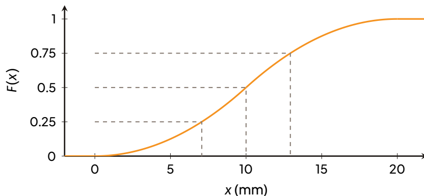
Cumulative distribution function of X , with the median and the quartiles read off.
