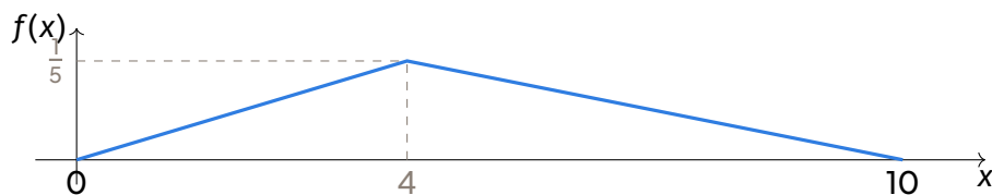
Triangular density with mode at x = 4 .
