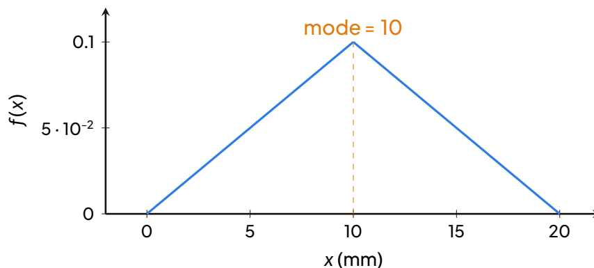
Probability density function of daily rainfall X (triangular model).
