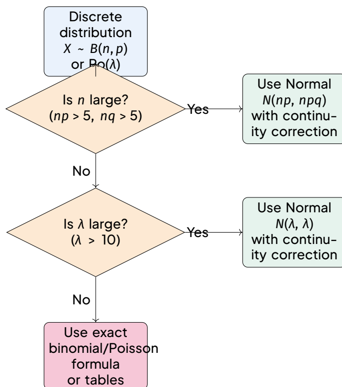
Decision flowchart for choosing the normal approximation.
