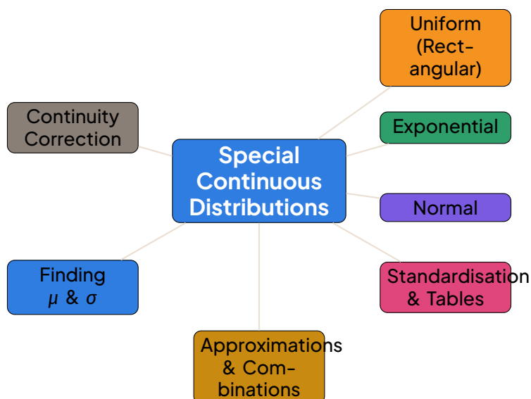
Mind map of Special Continuous Distributions
