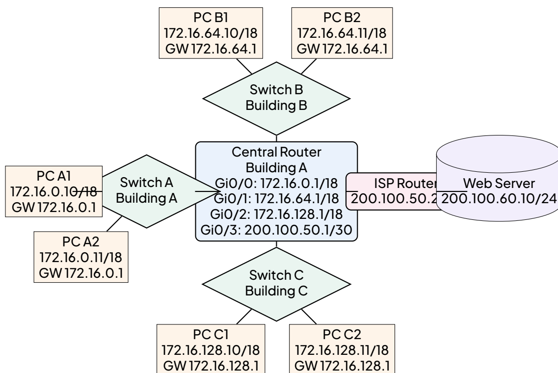
Topology for Lycée Bilingue de Bafoussam network simulation
