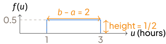
Probability density function of U \sim \text{Uniform}[1, 3]
