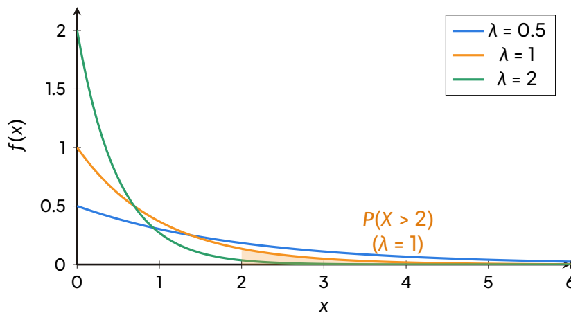
Densities of \text{Exp}(\lambda) for \lambda = 0.5, 1, 2 . Larger \lambda means faster decay and shorter typical waiting times. The shaded region is P(X > 2) = e^{-2} for \lambda = 1 .
