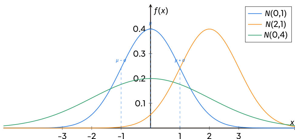
Normal curves: N(0,1) (blue), N(2,1) (orange), N(0,4) (green). The blue curve shows inflection points at \mu \pm \sigma .
