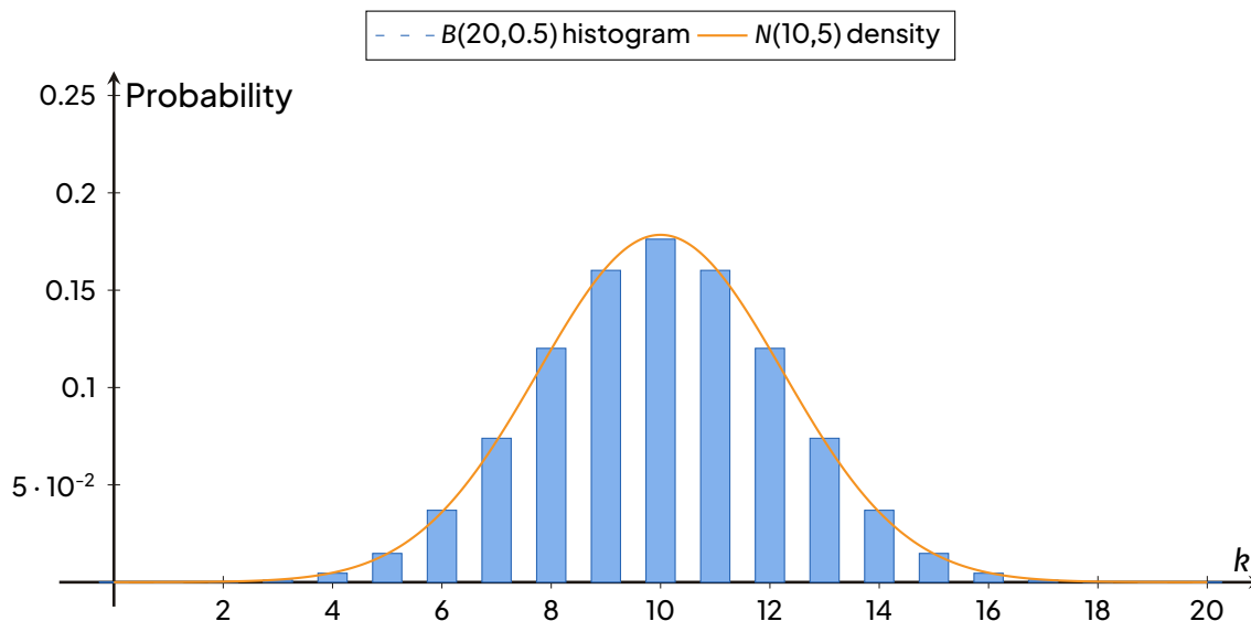
Histogram of B(20, 0.5) with superimposed normal curve N(10, 5) . The fit is already good at n = 20 .
