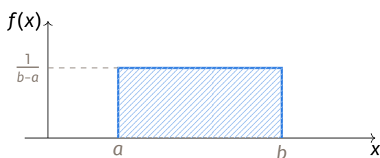
Density of the uniform distribution U(a, b) .
