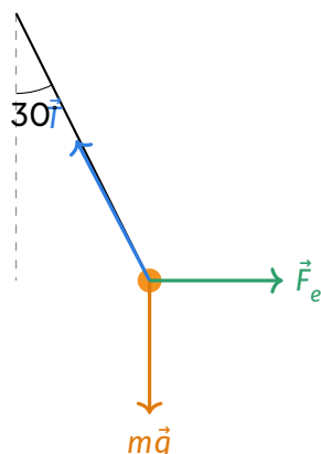
Equilibrium of the charged sphere under weight, tension and electrostatic force.
