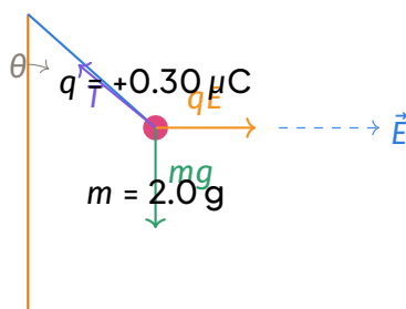
Free-body diagram of a charged pendulum in a uniform horizontal electric field.
