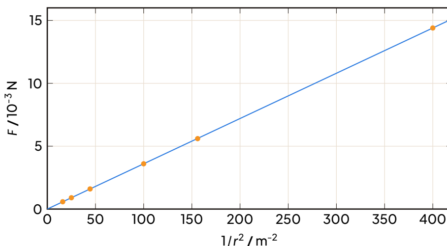
Graph of F against 1/r^2 : the points lie on a straight line through the origin, confirming the inverse-square law.
