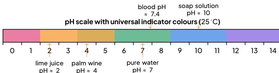
The pH scale with universal indicator colours and familiar examples.
