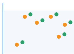
HCl (strong) only \text{H}_3\text{O}^+ and \text{Cl}^- ions
