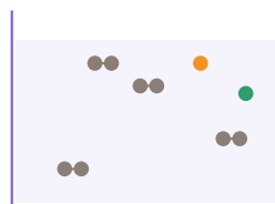
\text{CH}_3\text{COOH} (weak) mostly molecules, few ions
