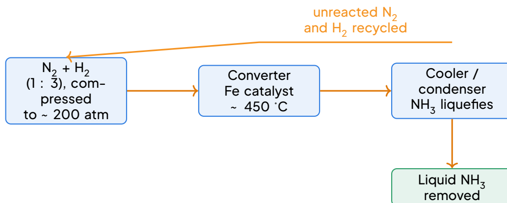
Flow diagram of the Haber process, with the recycle loop for unreacted gases.
