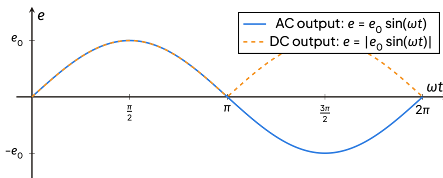
Output e.m.f. of the simple AC generator (sinusoid) and of the simple DC generator (rectified, pulsating) on the same axes.
