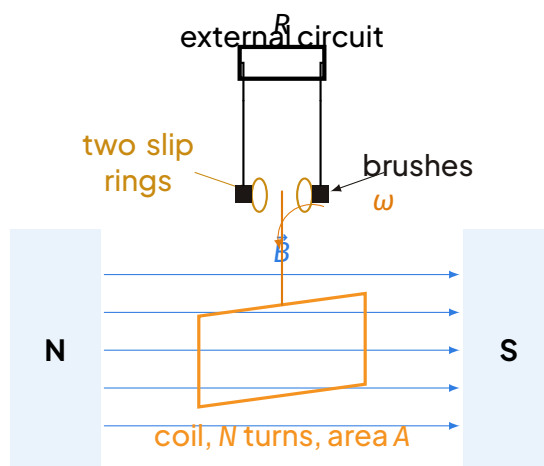
The simple AC generator: a coil rotating in a uniform field, connected to the external circuit through two slip rings and two brushes.
