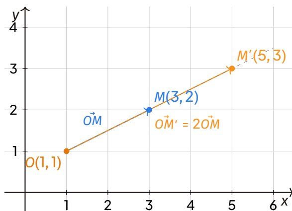
Homothety of centre O(1, 1) and ratio k = 2 : M(3, 2) \mapsto M'(5, 3) , with O, M, M' collinear.
