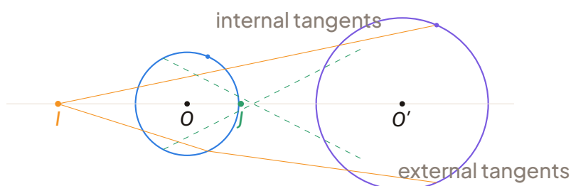
Two circles with R' \neq R : the external centre of similitude I (external tangents) and the internal centre J (internal tangents), both on the line of centres (OO') .
