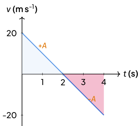
Velocity-time graph of the ball: gradient -g = -10 \text{ m s}^{-2} .
