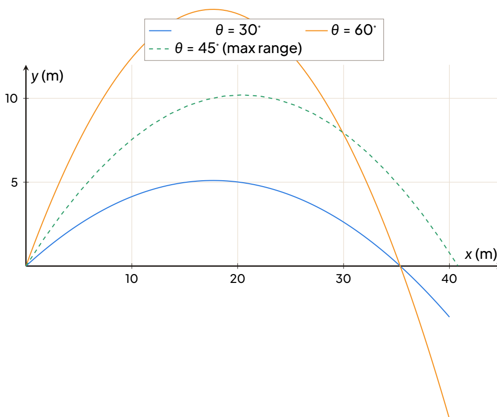
Trajectories for u = 20 \text{ ms}^{-1} at 30^\circ , 45^\circ and 60^\circ ( g = 9.8 ). The 30^\circ and 60^\circ trajectories have the same range; 45^\circ gives the maximum range.
