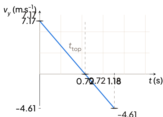
Vertical component of velocity during the flight of the optimal free kick ( \theta = 21^\circ ).
