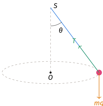
Forces on the bob of a conical pendulum.
