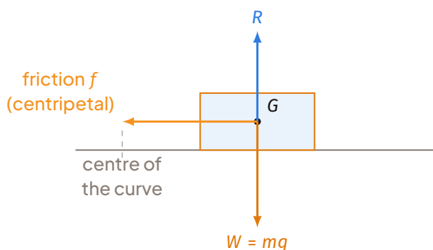
Free-body diagram of a vehicle on a flat curve (viewed from behind). Friction f towards the centre supplies the centripetal force; vertically R = mg .
