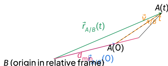
Closest approach: perpendicular from origin to relative path
