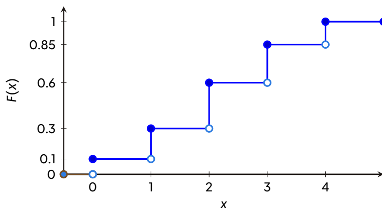
Cumulative distribution function of X (closed dots included, open dots excluded).
