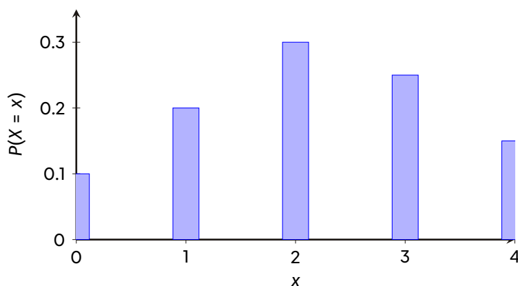
Probability mass function of the hourly number of withdrawals X .
