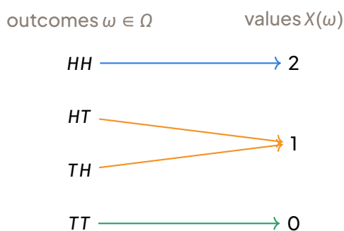
The random variable X as a function from \Omega to \mathbb{R} : HT and TH both map to 1.
