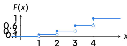
Cumulative distribution function for Exercise 5
