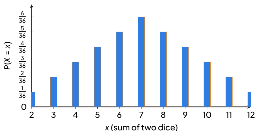
Probability histogram of X = \text{sum of two fair dice} : a symmetric triangular distribution peaking at x = 7 .
