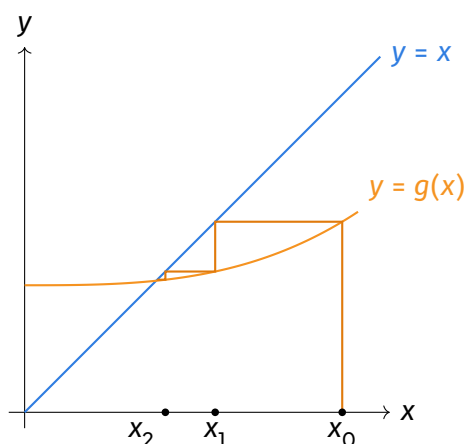
Staircase diagram: the iterates converge to the intersection of y = x and y = g(x) .
