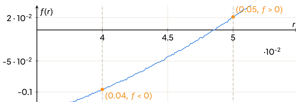
Graph of f(r) showing the sign change on [0.04, 0.05] .
