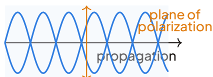
Plane polarized wave: vibrations confined to one plane
