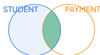
LEFT JOIN: all students
