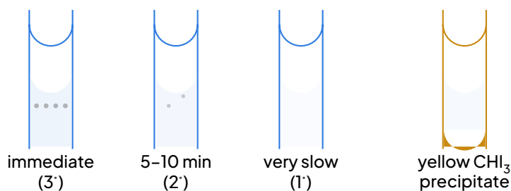
Schematic observations: Lucas turbidity for 3°, 2° and 1° alcohols, and the yellow iodoform precipitate.
