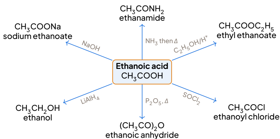
Reaction map centred on ethanoic acid.
