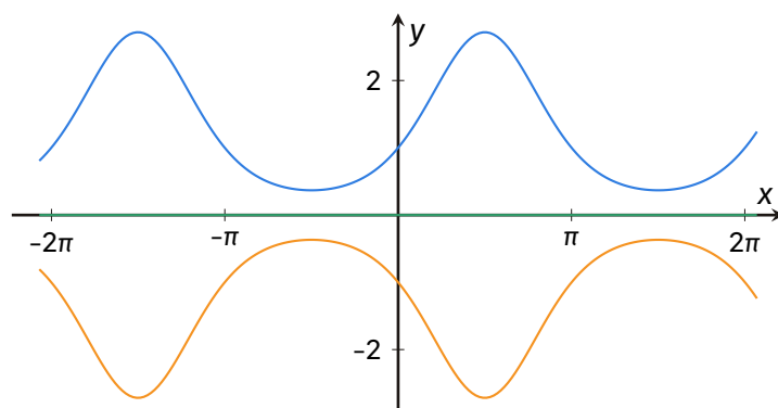
Curves y = e^{\sin x} (blue), y = -e^{\sin x} (orange), y = 0 (green)
