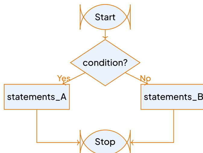
Flowchart for IF...ELSE (two-way selection). Both branches rejoin after the statements.
