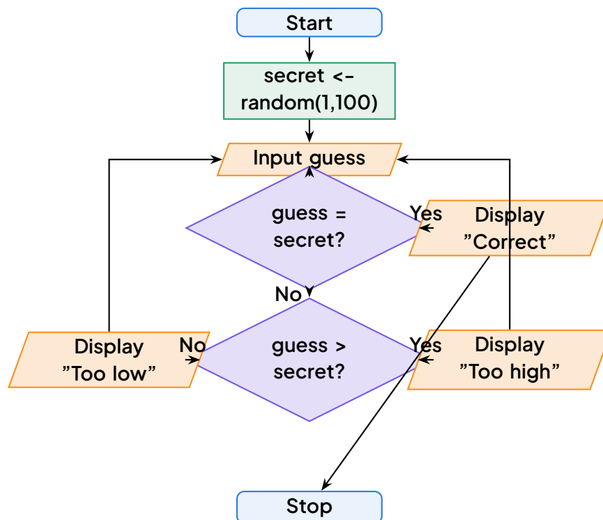
Flowchart for number-guessing game
