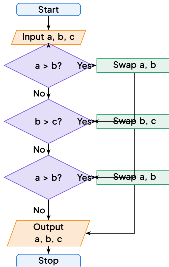
Flowchart for sorting three numbers in ascending order
