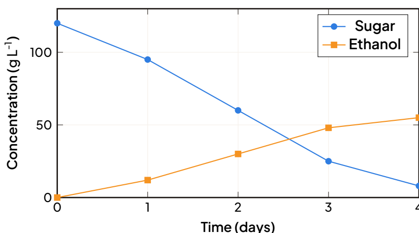
Sugar consumption and ethanol production during alcoholic fermentation.
