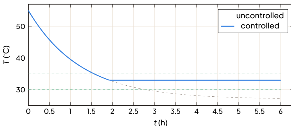
Controlled vs uncontrolled cooling; dashed green lines delimit the target band.
