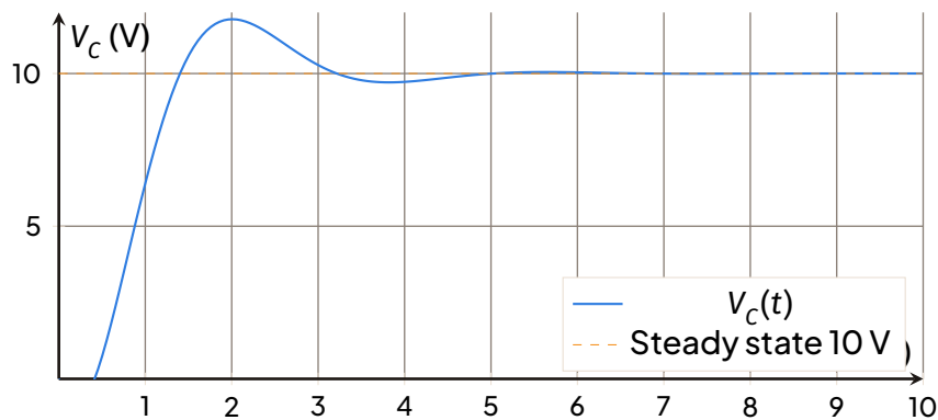
Underdamped voltage across the capacitor in a series RLC circuit.
