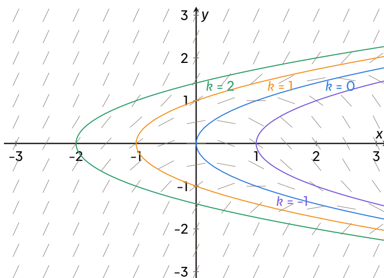
Direction field for \frac{dy}{dx} = y^2 - x with isoclines x = y^2 - k (parabolas). Along each parabola all segments have the same slope k .
