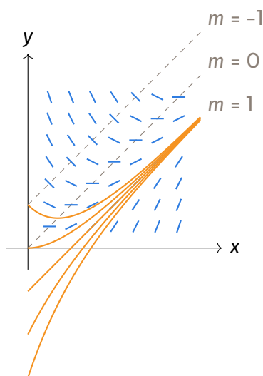
Direction field and integral curves for \frac{dy}{dx} = x - y .
