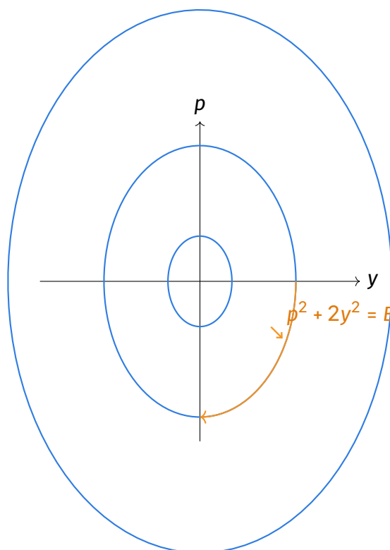
Phase plane trajectories for p \, dp/dy = -2y (ellipses p^2 + 2y^2 = E ).
