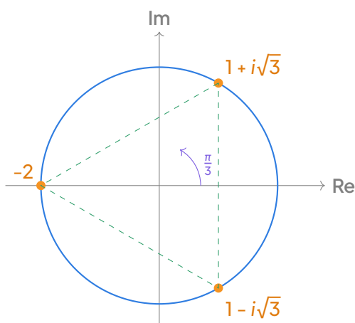
The cube roots of -8 : vertices of an equilateral triangle on the circle |z| = 2 .
