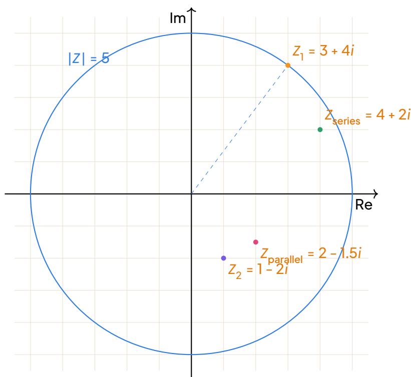
Argand diagram: the locus |Z| = 5 (circle, centre O , radius 5) and the four impedances. Only Z_1 lies on the circle.
