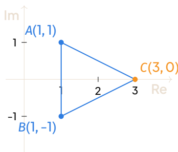
Triangle formed by the images of the three roots of P .
