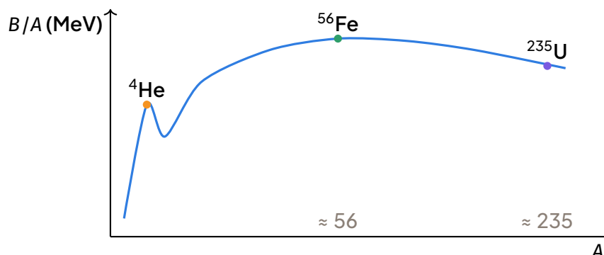
Binding energy per nucleon versus nucleon number (Aston curve).
