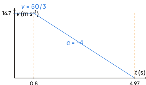
Velocity–time graph for the emergency stop.
