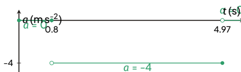
Acceleration–time graph. a = 0 during reaction, a = -4 \text{ m s}^{-2} during braking, a = 0 after stop.
