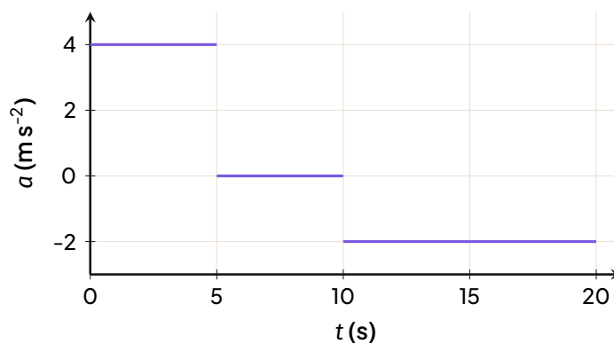
Acceleration-time graph of the particle.
