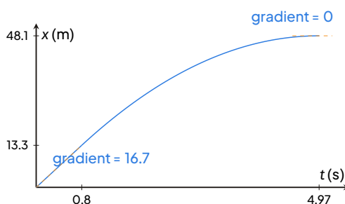
Displacement–time graph. Gradient at t = 0 is u = 16.7 \text{ m s}^{-1} ; gradient at stop is 0.
