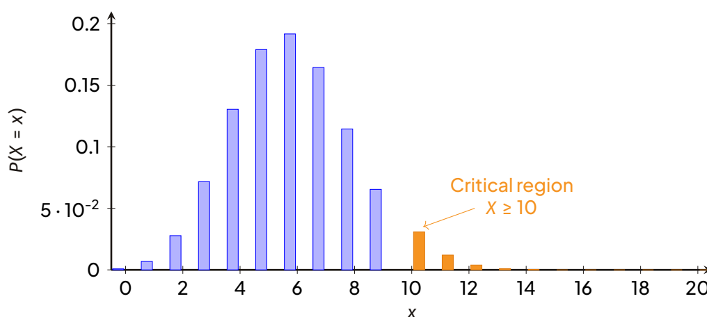
Distribution B(20, 0.3) under H_0 . The orange bars form the upper-tail critical region X \geq 10 for a test at the 5% level (actual level 0.0480).
