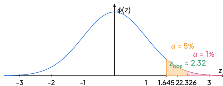
Standard normal density showing critical regions for one-tailed tests at 5% ( z > 1.645 ) and 1% ( z > 2.326 ), and the observed statistic z_{\text{obs}} \approx 2.32 for Test 1.
