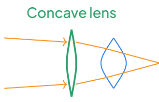
Myopia corrected
