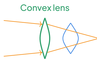
Hypermetropia corrected
