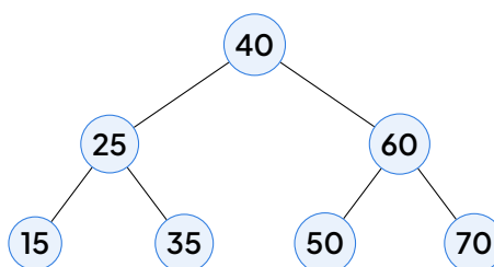
BST after inserting 40, 25, 60, 15, 35, 50, 70.
