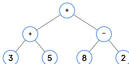
Expression tree for (3 + 5) \times (8 - 2) .
