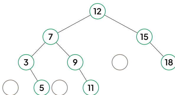
BST built from the insertion order 12, 7, 15, 3, 9, 18, 11, 5.
