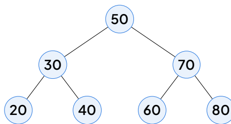
BST after inserting 50, 30, 70, 20, 40, 60, 80.
