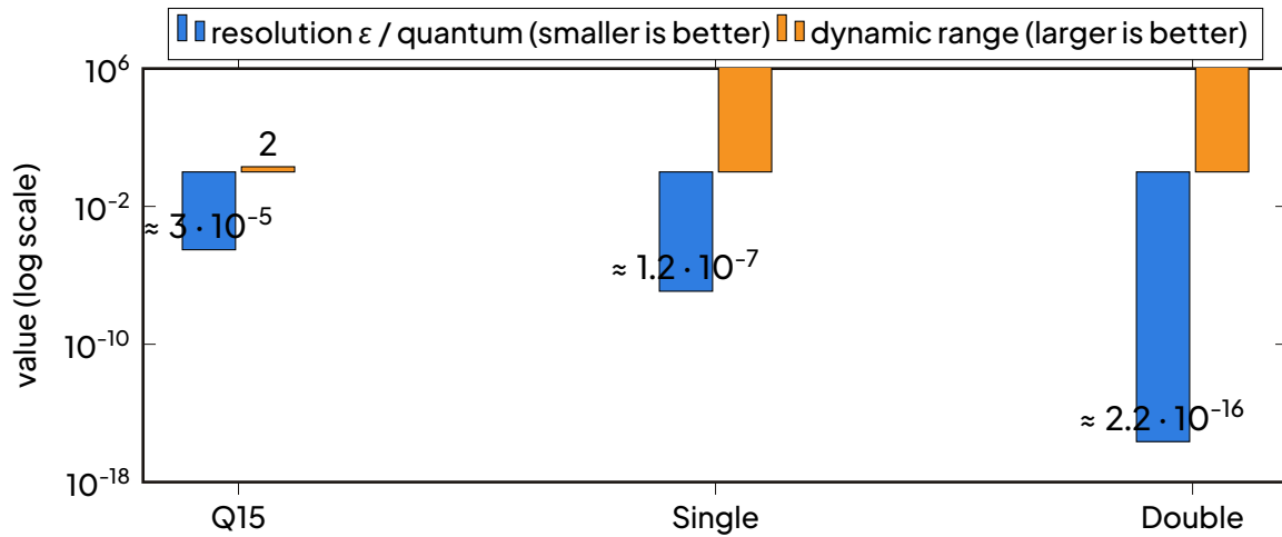
Comparison of Q15 fixed-point, IEEE 754 single and double precision: resolution (machine epsilon or quantum) and dynamic range (ratio of largest to smallest positive normal value, log scale).
