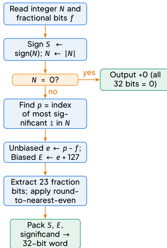
Flowchart of the fixed-point (Qf) to IEEE 754 binary32 conversion routine.
