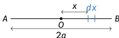
Element of a uniform rod for moment of inertia calculation.
