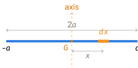
Rod with element of length dx at distance x from the central axis.
