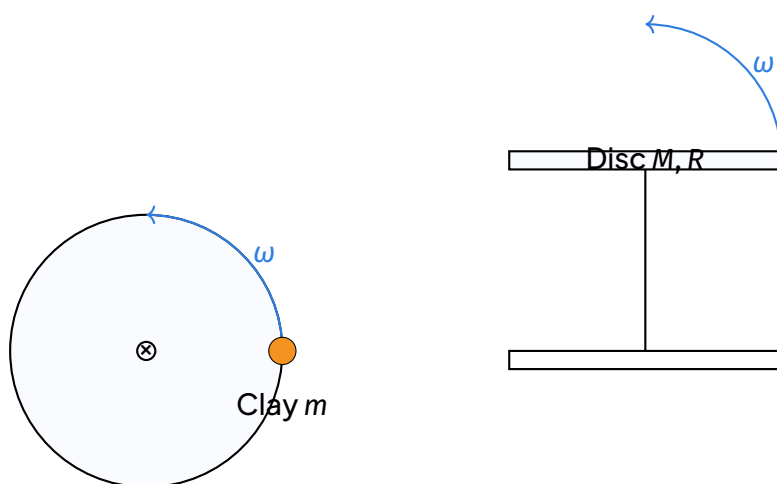
Top view (left) and side view (right) of the potter's wheel. The clay lump is dropped onto the rim.
