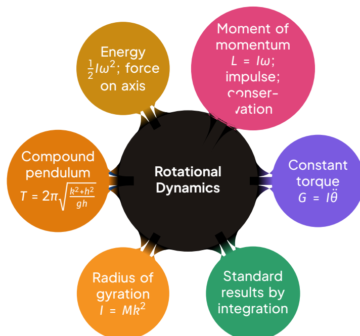
Mind map of the chapter Rotational Dynamics.
