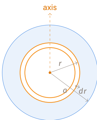
Disc divided into concentric rings of radius r and width dr .
