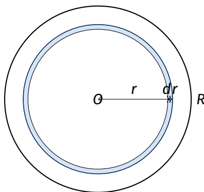
Concentric ring element for a uniform disc.
