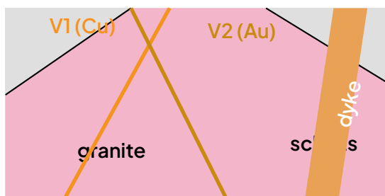
Cross-section: granite in schists, veins V1 and V2, dolerite dyke.
