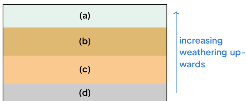
Schematic lateritic profile, Minim-Martap.
