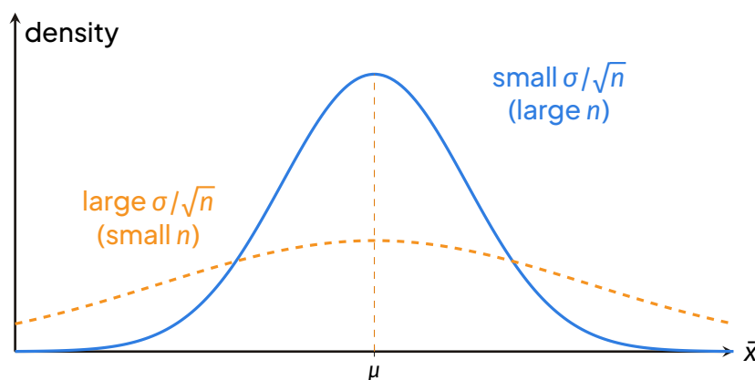
Sampling distribution of \bar{X} : normal curves centred on the population mean \mu . The spread (standard error \sigma/\sqrt{n} ) decreases as n increases.
