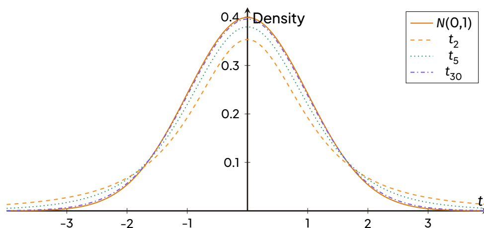
Probability density functions of t -distributions with \nu = 2, 5, 30 and the standard normal N(0, 1) . As \nu increases, the t -distribution approaches the normal.
