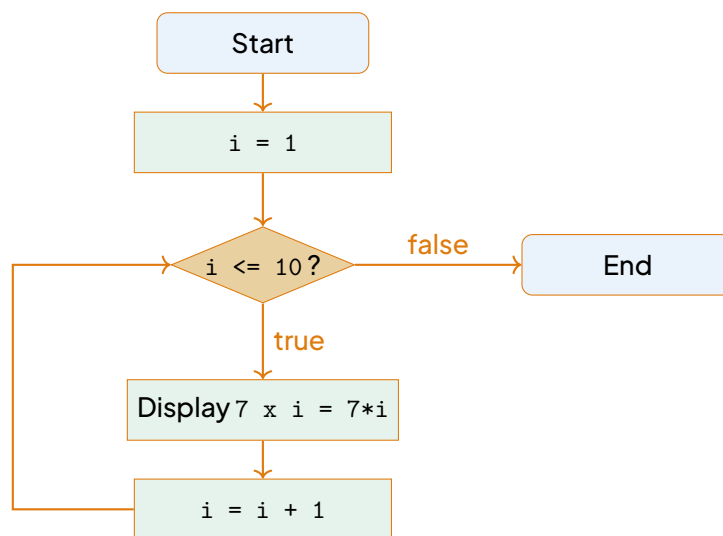
Flowchart of a for loop printing the multiplication table of 7, for i from 1 to 10.
