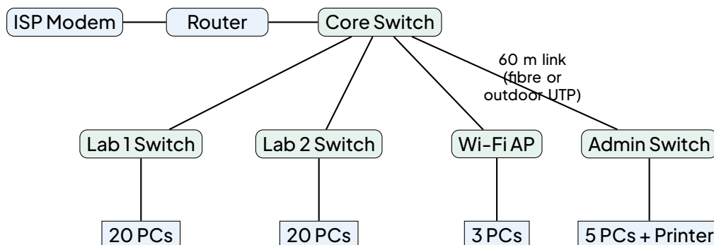
Proposed tree topology for Garrison Secondary School.
