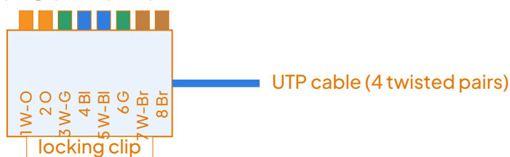
RJ45 plug (pins up, clip down)
