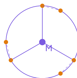
\Delta -[M(en) 3 ] 3+ Right-handed propeller
