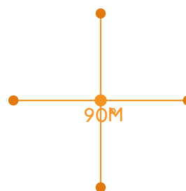
Square Planar (CN=4) e.g. [\text{Pt}(\text{NH}_3)_2\text{Cl}_2]
