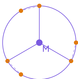
\Lambda -[M(en) 3 ] 3+ Left-handed propeller
