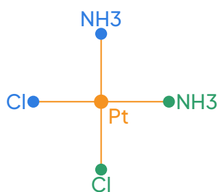
cis -[Pt(NH 3 ) 2 Cl 2 ] Cl-Pt-Cl = 90° Dipole moment ≠ 0
