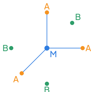
fac -[MA 3 B 3 ] A's on one face
