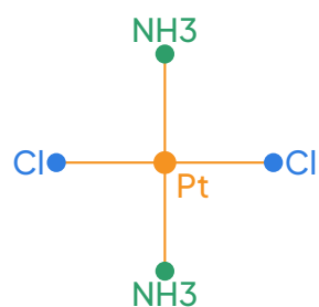
trans -[Pt(NH 3 ) 2 Cl 2 ] Cl-Pt-Cl = 180° Dipole moment = 0
