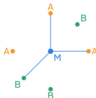
mer -[MA 3 B 3 ] A's in a meridian
