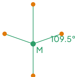
Tetrahedral (CN=4) e.g. [\text{CoCl}_4]^{2-}
