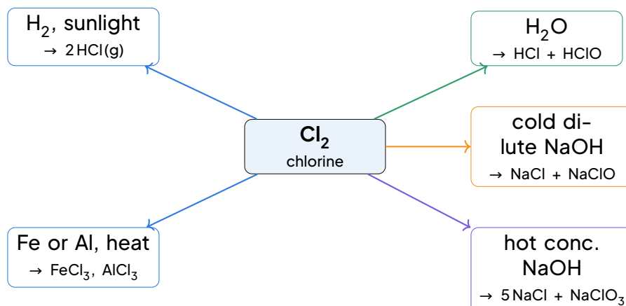
Summary flow diagram of the principal reactions of chlorine.
