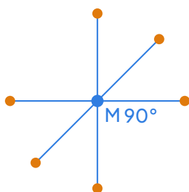
Octahedral (CN=6) e.g. [\text{Fe}(\text{H}_2\text{O})_6]^{2+}
