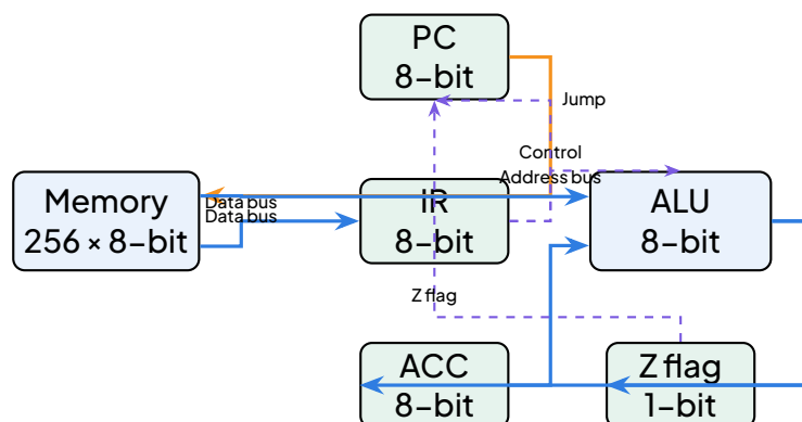
CamCPU-1 Von Neumann architecture: single mem- ory for program and data, shared address/data buses.
