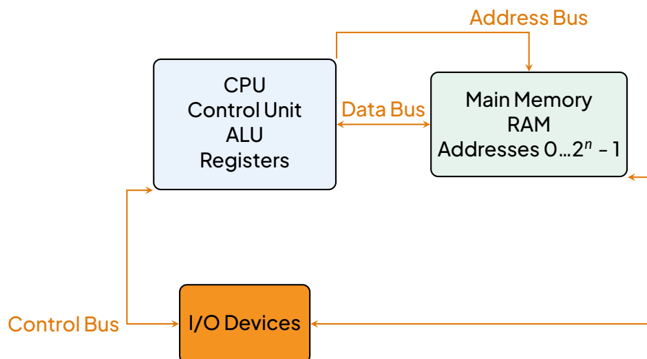
Von Neumann model: CPU, Memory, I/O connected by three buses.
